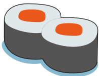
MAKI
