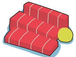
SASHIMI
